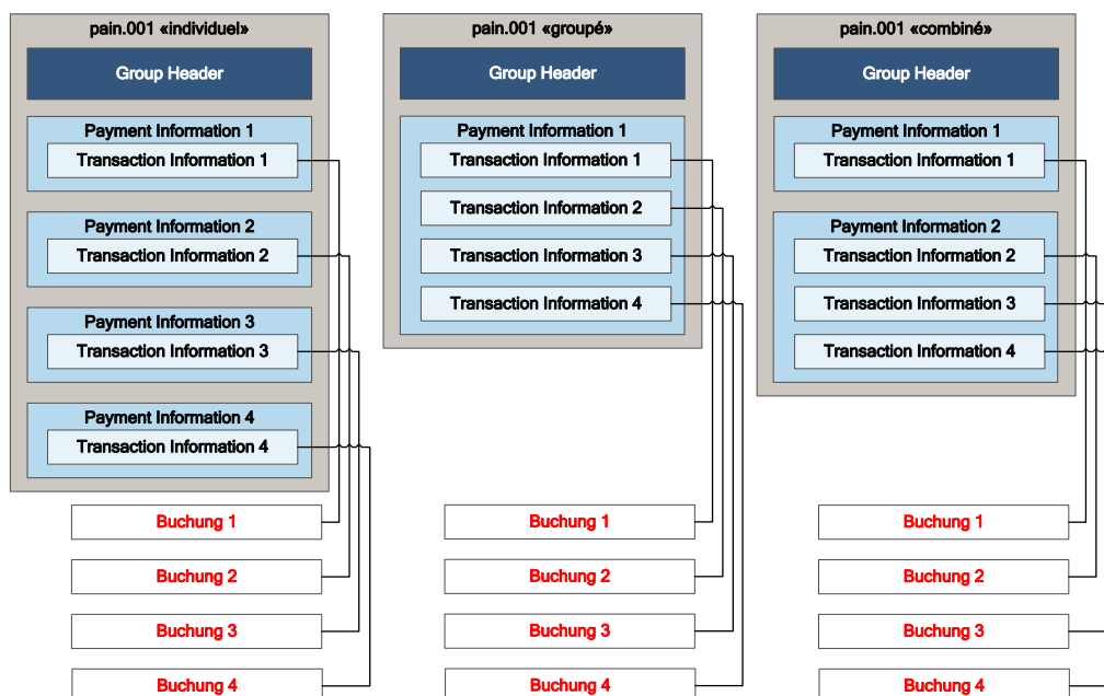
Illustration 7: Batch Booking FALSE
