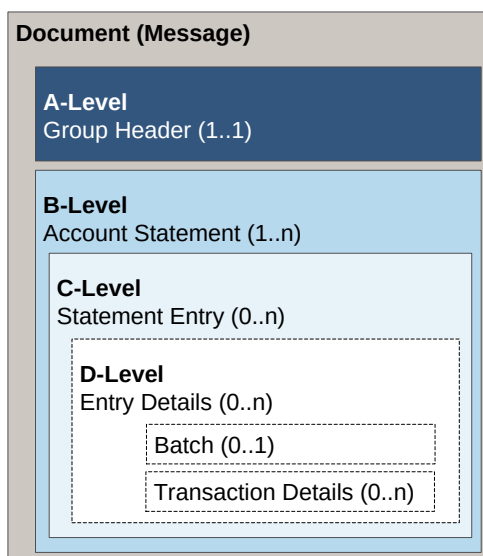
Illustration 5: Structure des messages Cash Management
