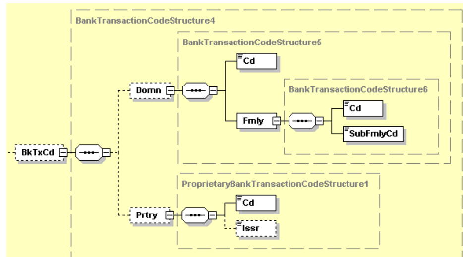
Illustration 11: Bank Transaction Code
