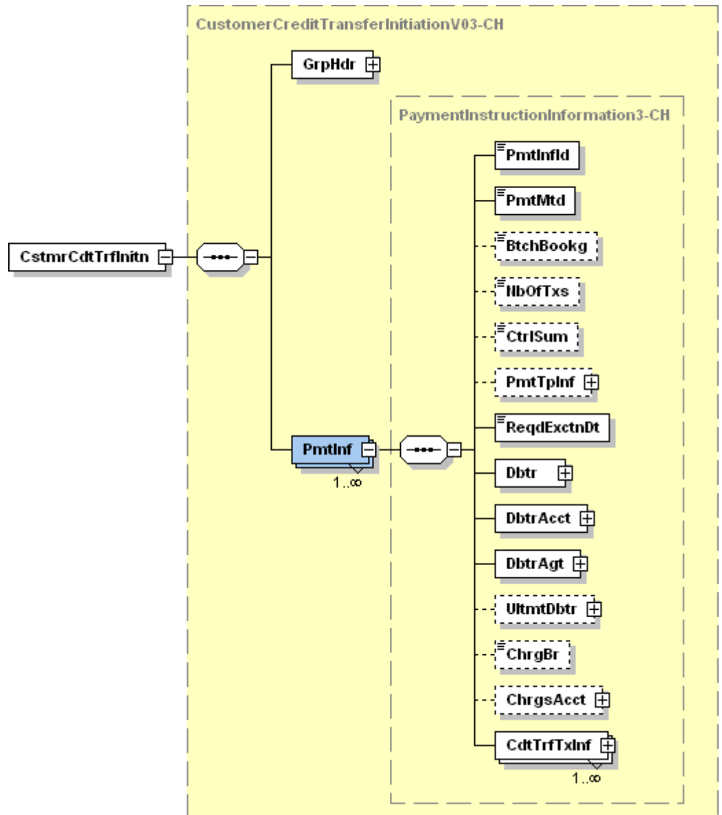
Illustration 8: Payment Information (PmtInf)
