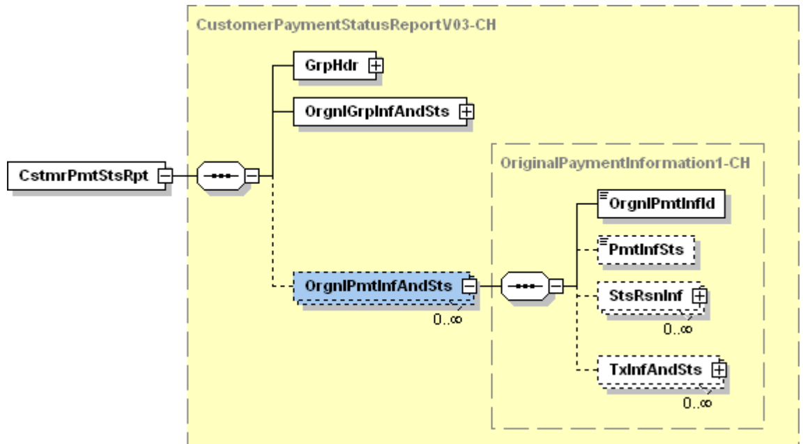
Illustration 14: Original Payment Information And Status (OrgnPmtInfAndSts)
