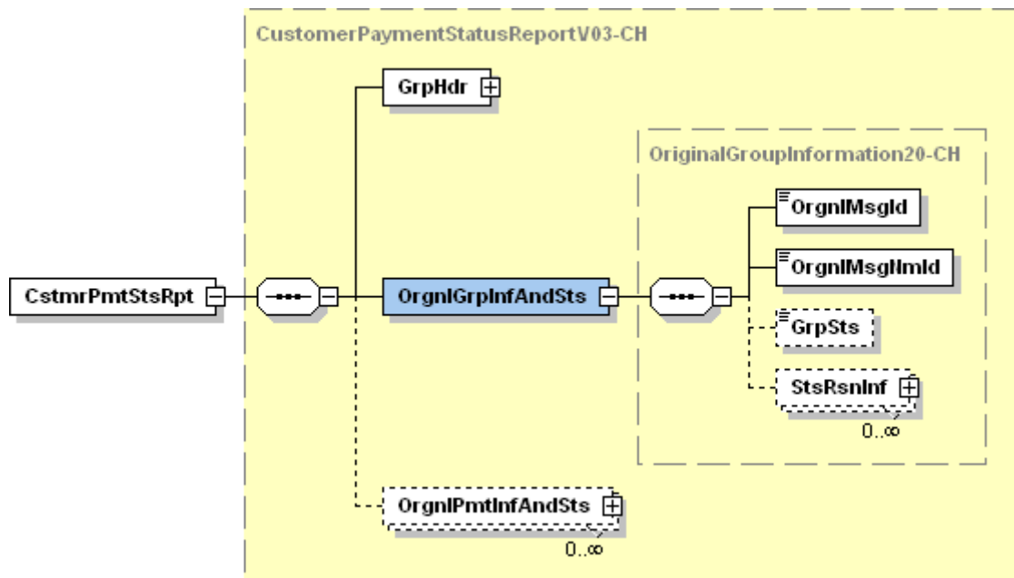
Illustration 13: Original Group Information And Status (OrgnlGrpInfAndSts)
