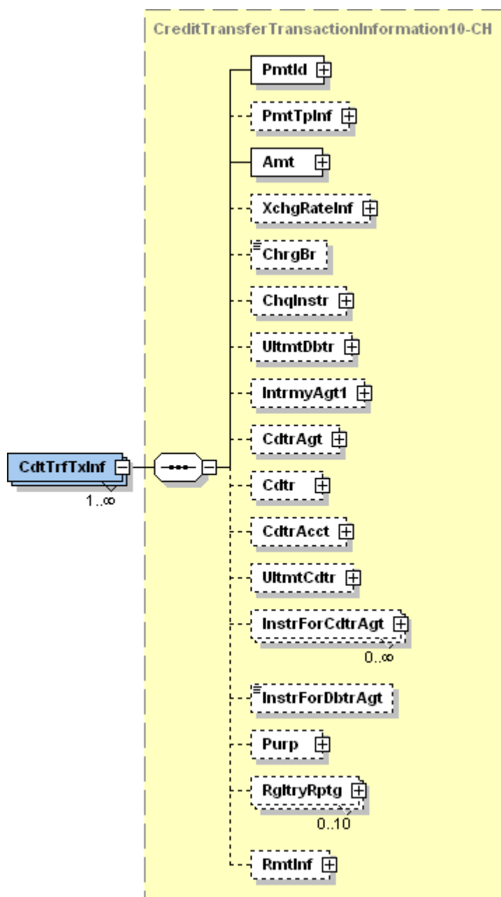
Illustration 9: Credit Transfer Transaction Information (CdtTrfTxInf)
