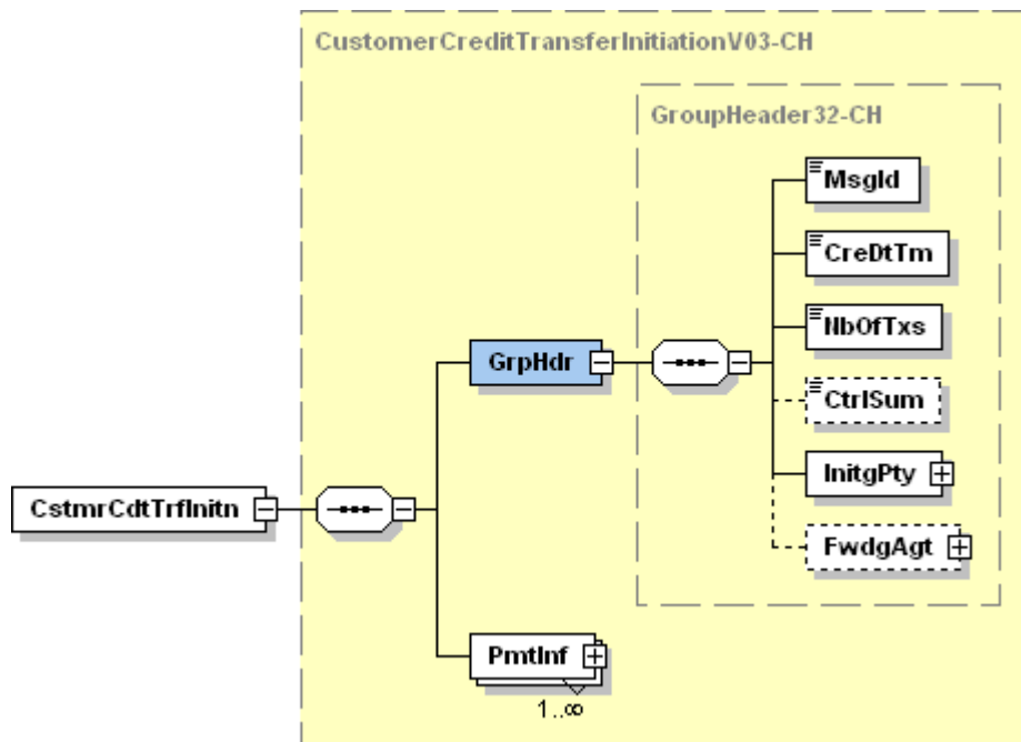
Illustration 7: Group Header (GrpHdr)
