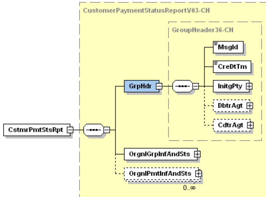
Illustration 12: Group Header (GrpHdr)
