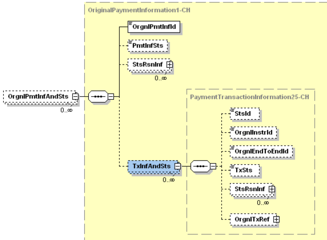
Illustration 15: Transaction Information And Status (TxInfAndSts)
