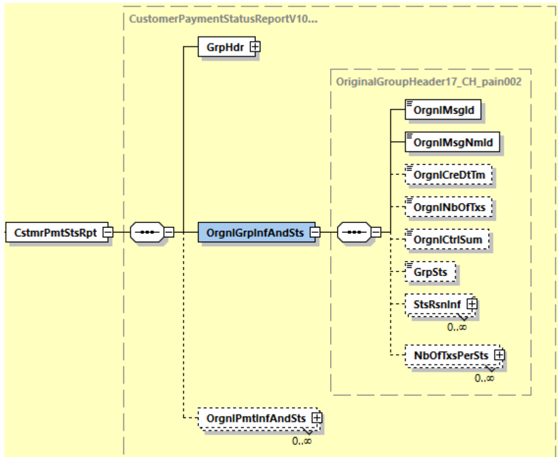
Illustration 10: Original Group Information And Status (OrgnlGrpInfAndSts)
