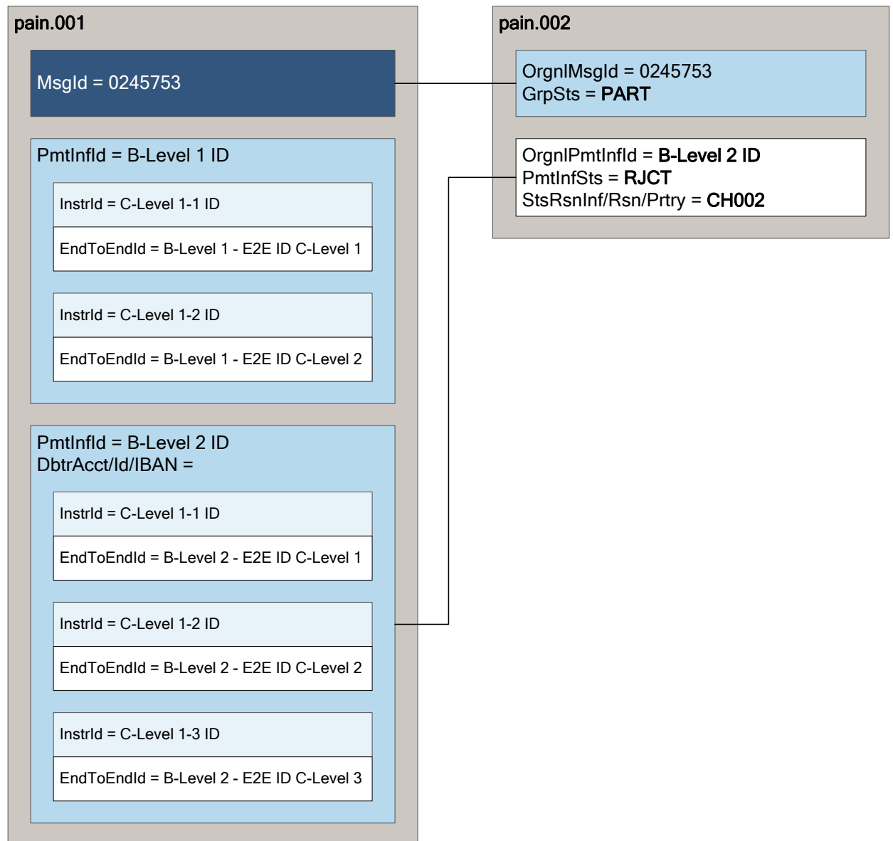
Illustration 15: Exemple Status Report Rejected B-Level
