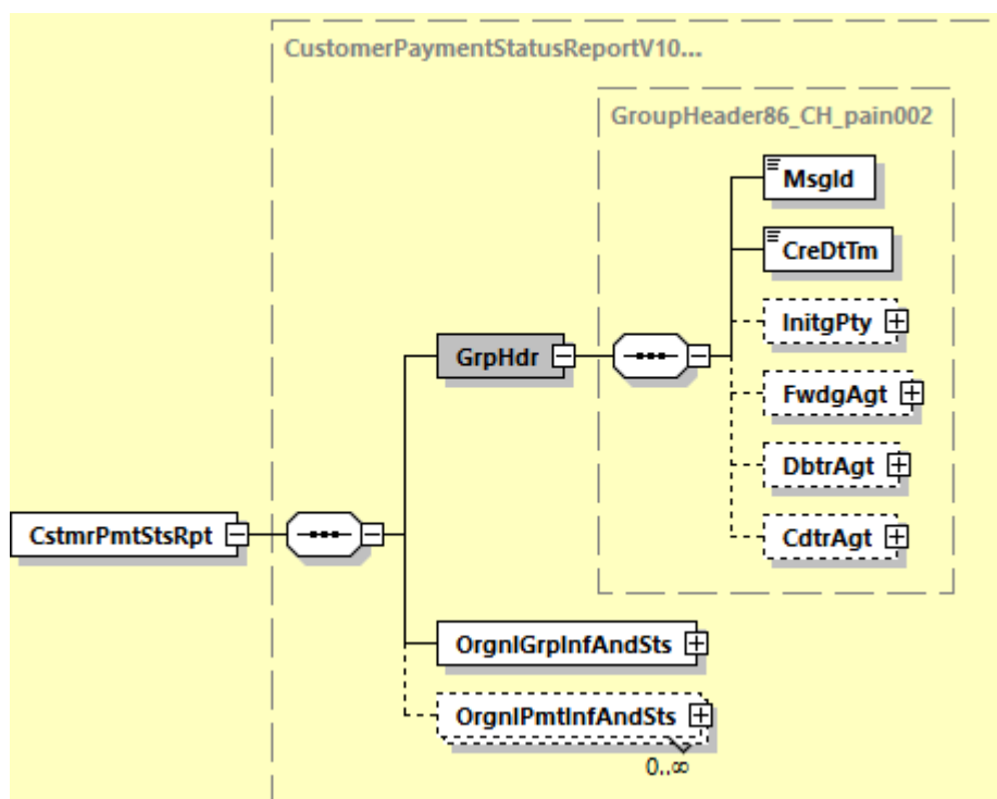
Illustration 9: Group Header (GrpHdr)
