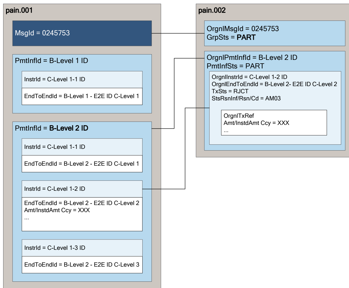
Illustration 16: Exemple Status Report Rejected C-Level
