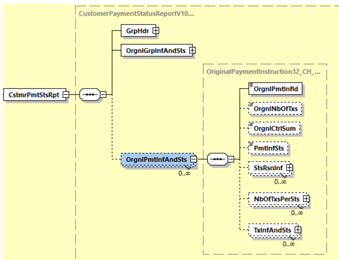
Illustration 11: Original Payment Information And Status (OrgnlPmtInfAndSts)
