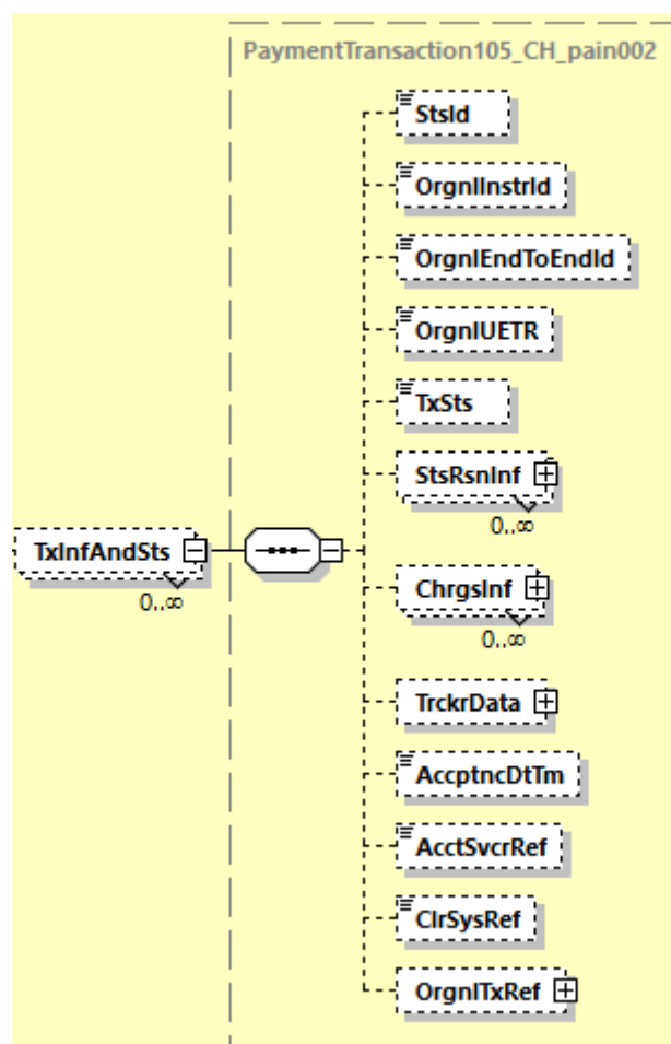
Illustration 12: Transaction Information And Status (TxInfAndSts)
