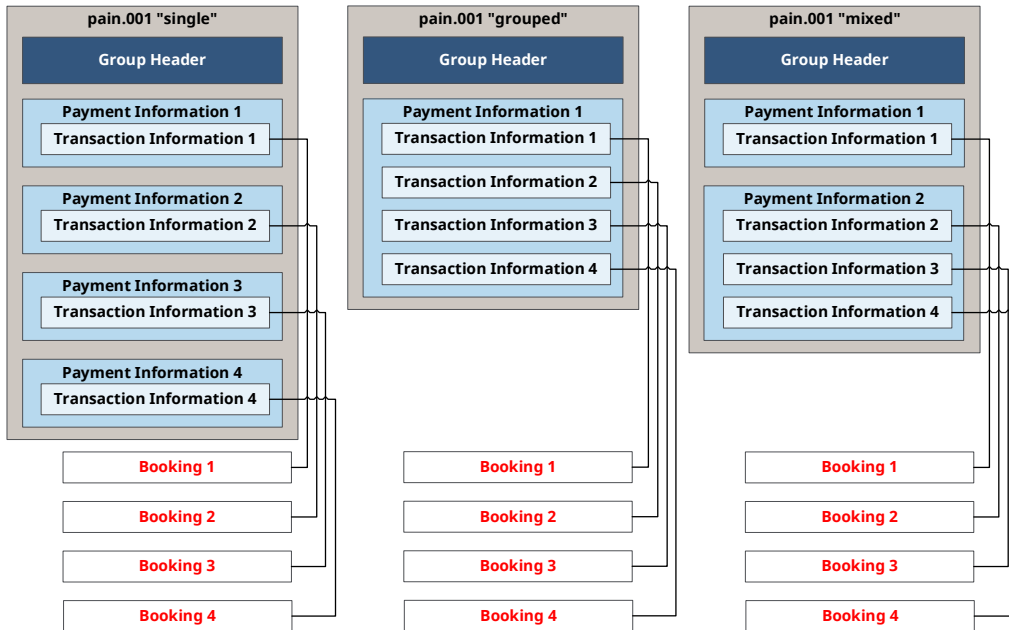
Figure 3: Batch Booking FALSE
