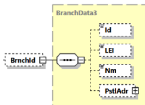
Figure 6: Additional data elements for the identification of branches of financial institutions (generic)
