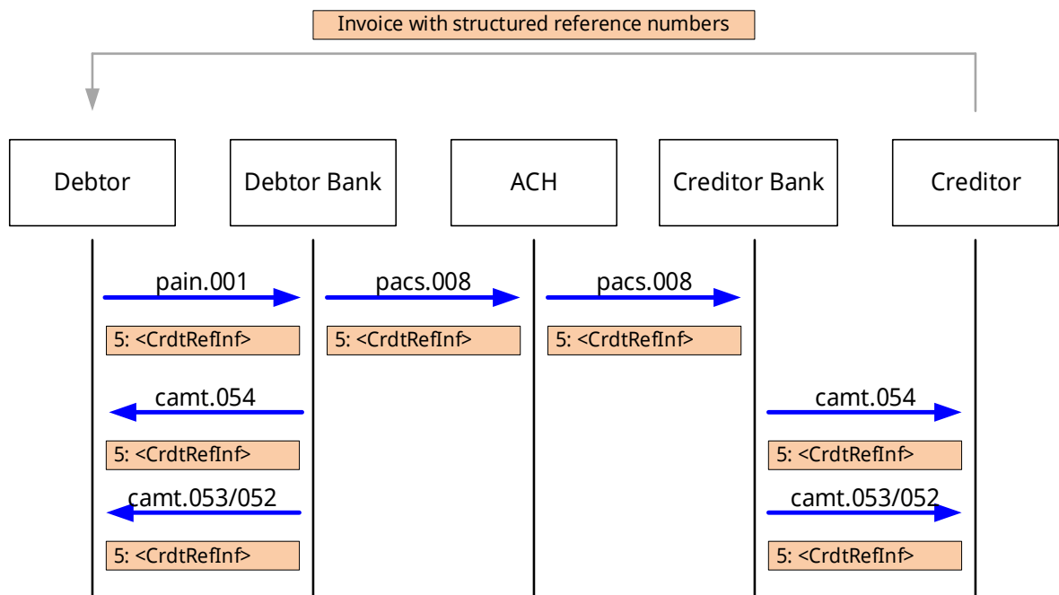
Figure 10: Structured reference in Credit Transfer (pain.001)
