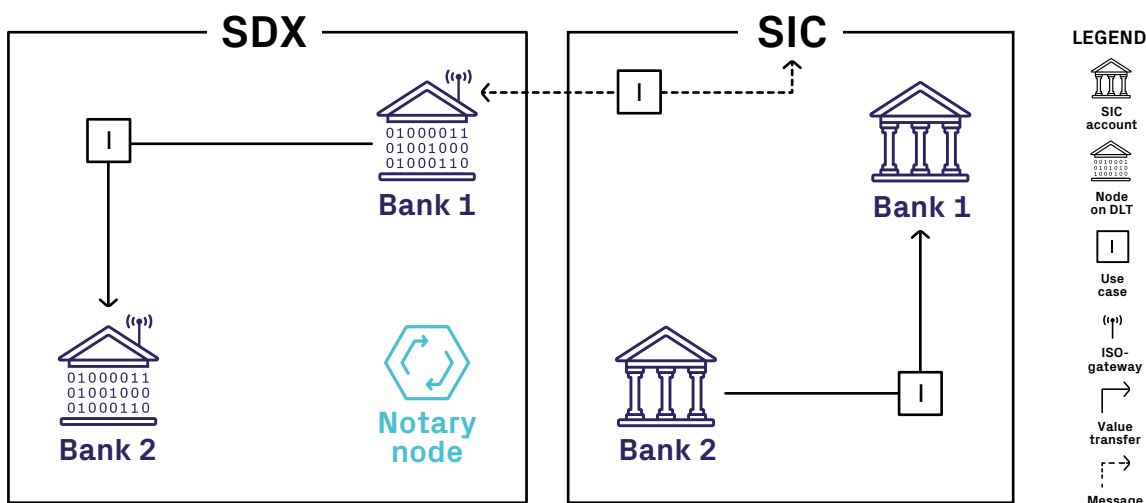
Graph 5: Solution design for DvP settlement in SIC balances (PoC2)
