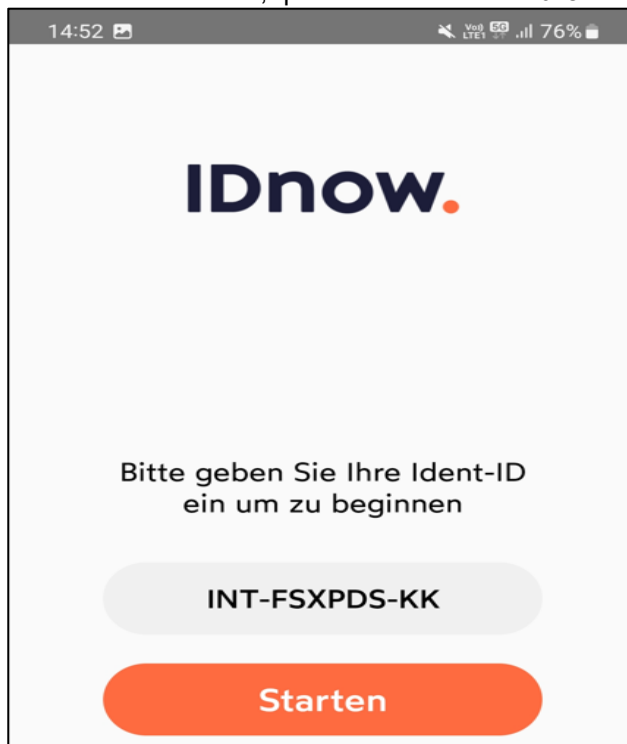
Figura 5, app IDnow
